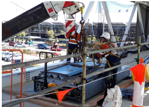
Modules-elevation maneuvers at Skybridge - Perth Airport (Australia)
