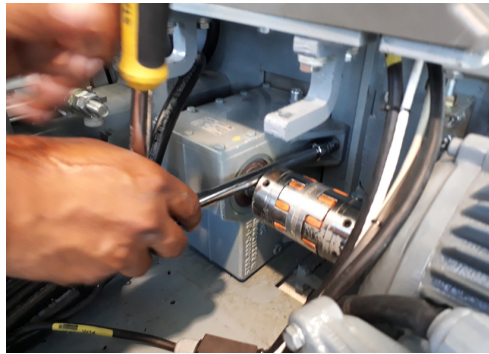
Adjustment and alignment of motor shaft coupling at Tocumen Airport (Panamá)
